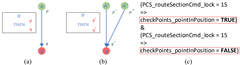
Figure 2: The implication in invariants.
