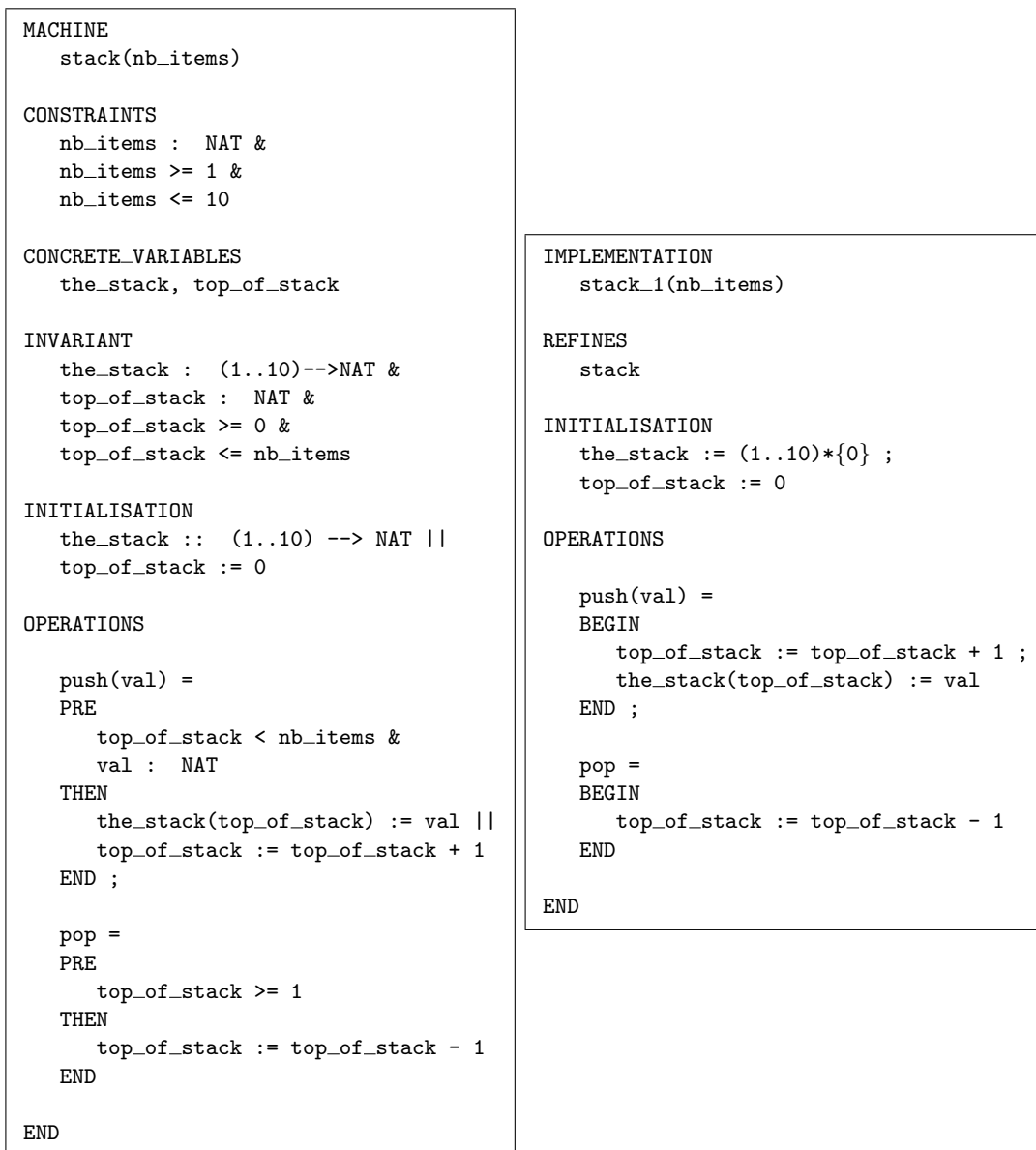
Figure 4.1: Specification and implementation of the stack component
